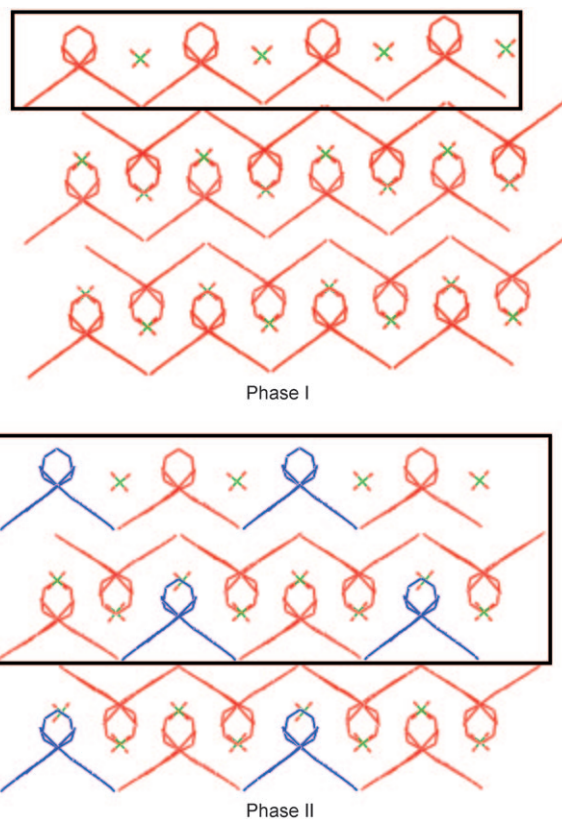
Figure 3. Representation of unit cell contents within the crystal packing of 1 in structural and spin phases I and II. The boxes represent the relative contents of the unit cell in each case but do not represent the true unit cell. The unit cell contents viewed from different orientations are shown in the Supporting Information.
